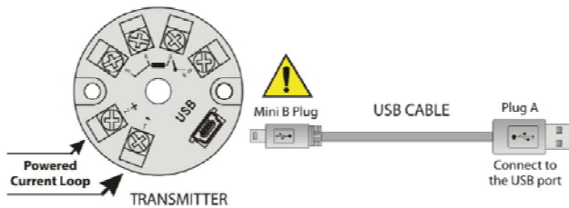
USB Cable Connection
