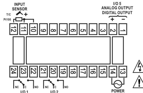
Figure 1 – Controller electrical connections
